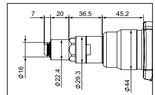
Nose piece access dimensions
